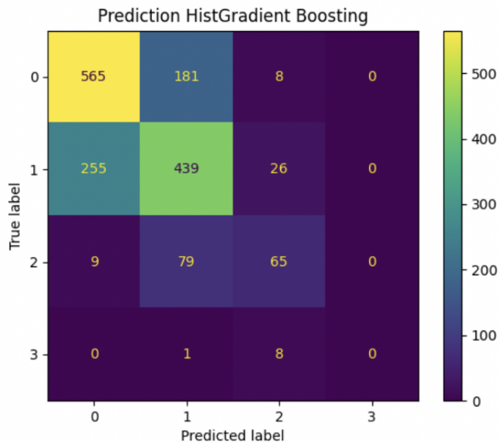
Figure 6: Confusion matrix of the seasonal-forecasts on the out-of-sample test set
