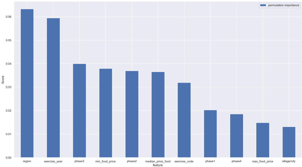
Figure 8: Permutation feature importance plot for Chad
